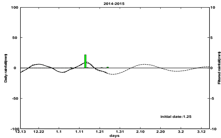
Fig. 1 Prediction (dashed line) and observation (solid line) of the 20—30-day rainfall over LYRV for the period from 1 into 50 days in the winter of 2014/2015 for ECAR model based on the principal components of the global low frequency the meridional wind anomaly of 850 hPa, and the bar represents the time series of the daily precipitation over LYRV(unit: mm) , initial date: January 25, 2015.
